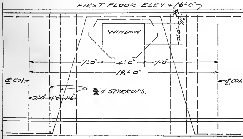
ELEVATION AT FF
